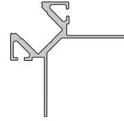
tile profiles outside corner from page 636
